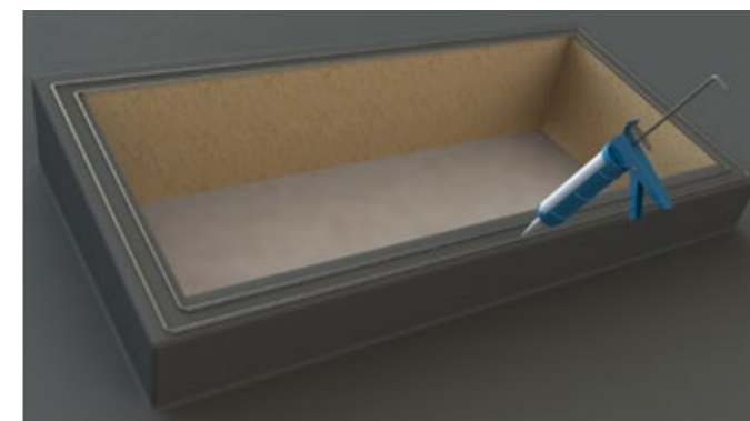
1 Run a continuous bead of sealant around the perimeter of the kerb for the frame to sit on.
