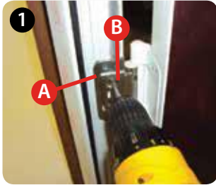
Loosen the 2 screws that clamp side plate (B) to frame plate (A)
