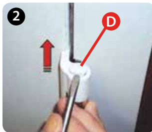
Carefully remove the top cap and with the 6mm socket tool rotate the hex pin (D).
