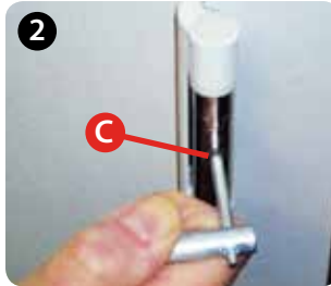
With the 4mm allen key tool loosen the socket screws (C) by about 1/3 of a turn.
