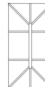
Maximum size Regular lantern as per this rafter layout 3000mm x 4000mm – can go up to 5000mm x 10000mm with additional rafters.
